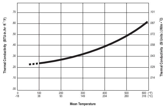
Thermal Efficiency (ASTM C 335)
